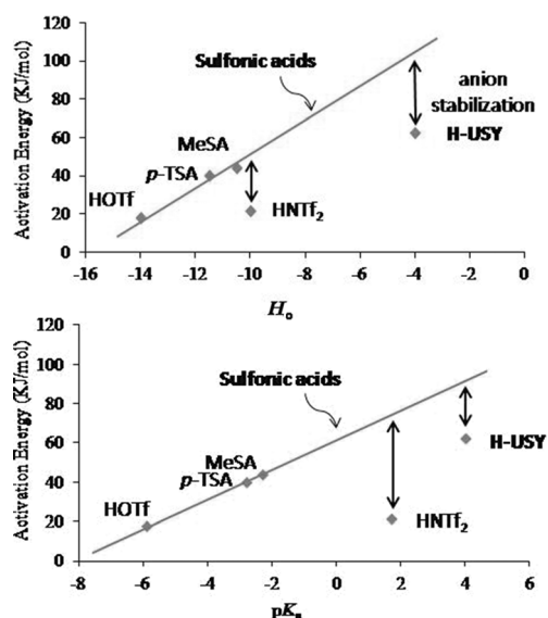
Figure 3. Activation energy–acidity values ( H_0 , top; pK_a , bottom) plot for different acids and H-USY zeolite. The activation energies of the reaction are calculated from the initial rate of the Meyer–Schuster rearrangement, by in situ NMR measurements (see Figure S3 for calculations). High catalytic loadings of H-USY (120 wt%) and HNTf 2 assure rapid formation of the ketone.
